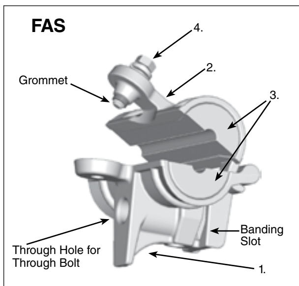
Through-Bolt Mounted
